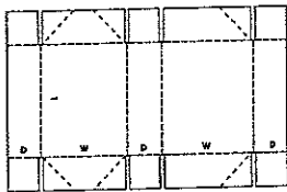
0760 Self Erecting Six Corner Tray
