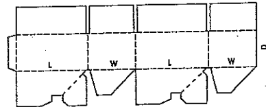
0711 Pre-glued Auto Bottom with RSC Top Flaps
