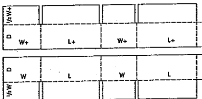
0320 Full Telescope Half Slotted Container (FTHS)
