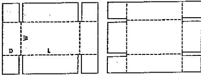
0301 Full Telescope Design Style Container (FTD)
